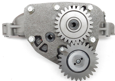
Lube Oil Pump Part No: USOP1757 OEM: 4309500
