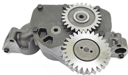
Lube Oil Pump Part No: USOP9499 OEM: 4309499
