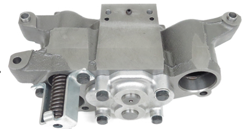
3406 / C15 / C18 Acert Oil Pump Part No: USOP8734 OEM: 4N8734
